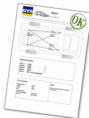
Frame rack
